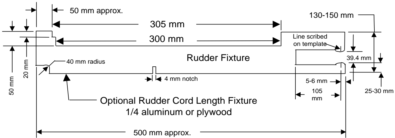
Keel and Rudder Measurement Fixtures Fig. 3.0
