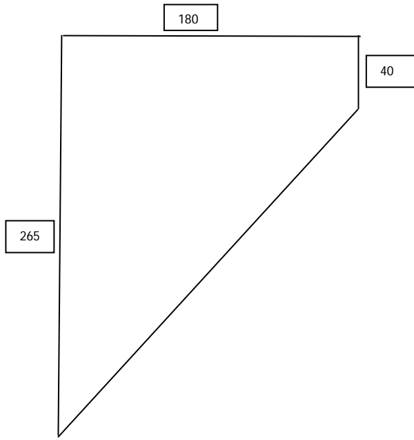
Diagram # 31 Farr 40 Headboard Dimensions (Not to Scale)
